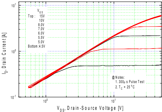
Figure 1. Output Characteristics
